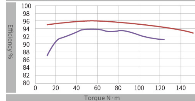
Efficiency curve chart
